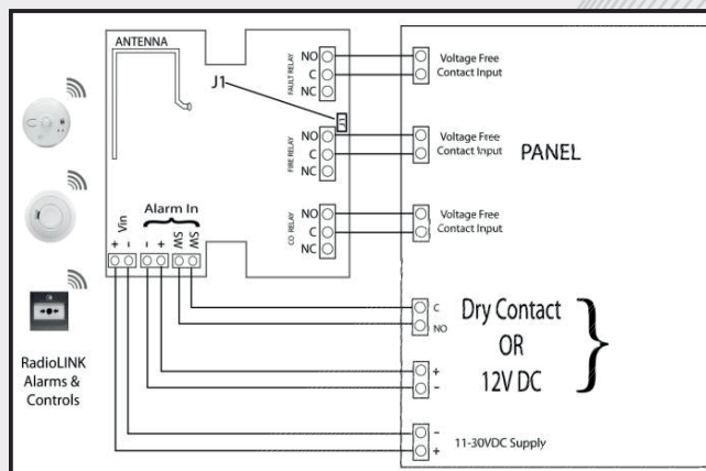
Security Panel wiring configuration
