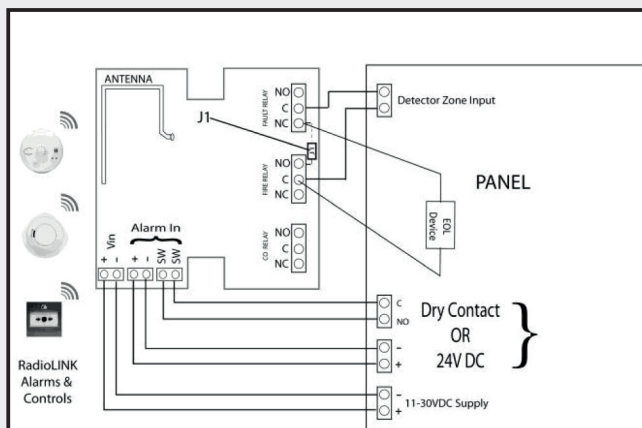
Typical Fire Panel wiring configuration
